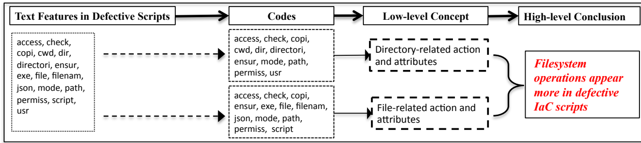
FIGURE 4 An example of how we use Strauss-Corbin Grounded Theory (SGT) to characterize defective IaC scripts.
