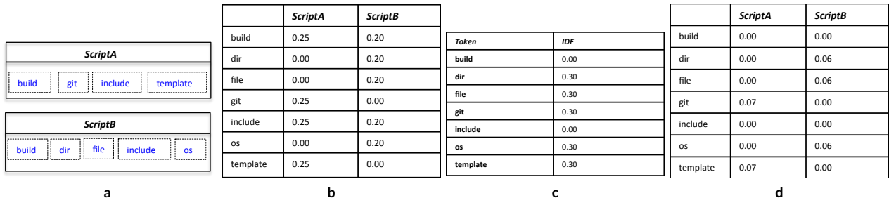
FIGURE 3 A hypothetical example to illustrate out feature vectorization technique using TF-IDF. Figure 3a presents the pre-processed tokens of two scripts: ScriptA and ScriptB. Figure 3b presents the TF values for both scripts. Figure 3c presents the IDF scores for the unique seven tokens. Finally, TF-IDF scores for each script and token is presented in Figure 3d.
