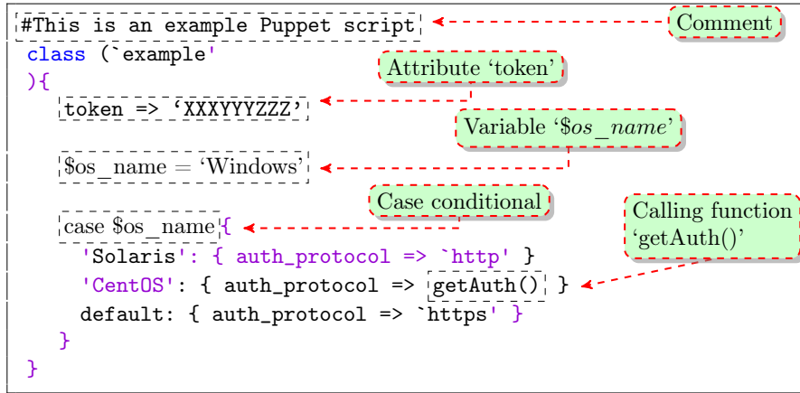
FIGURE 1 Annotation of an example Puppet script.
