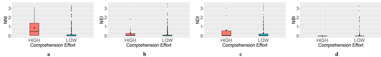
Figure 3: Navigation interval ( NNI ), edit interval ( NEI ), debugging interval ( NDI ), and build interval ( NBI ) values for sessions labeled as ‘High’ and ‘Low’. In ‘High’ sessions, programmers navigate and make edits at a significantly slower rate.
